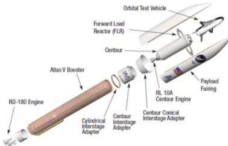
This ULA diagram depicts the Orbital Test Vehicle 1 space plane and its position atop the Atlas 5 (501) rocket Credit: United Launch Alliance.
